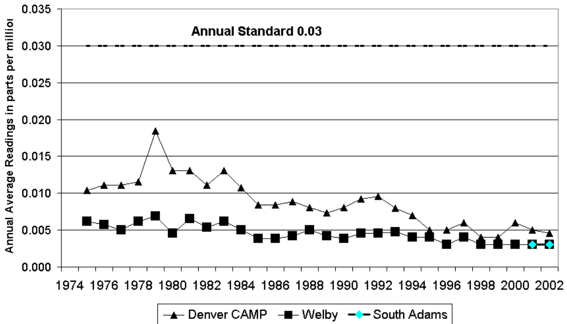
Figure 21 - Northern Front Range Nitrogen Dioxide Graphs
