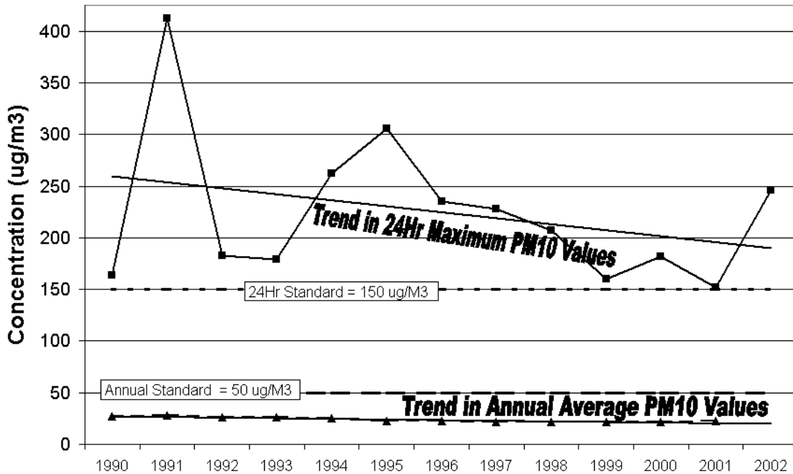
Figure 11 Statewide Ambient Trends - PM10
