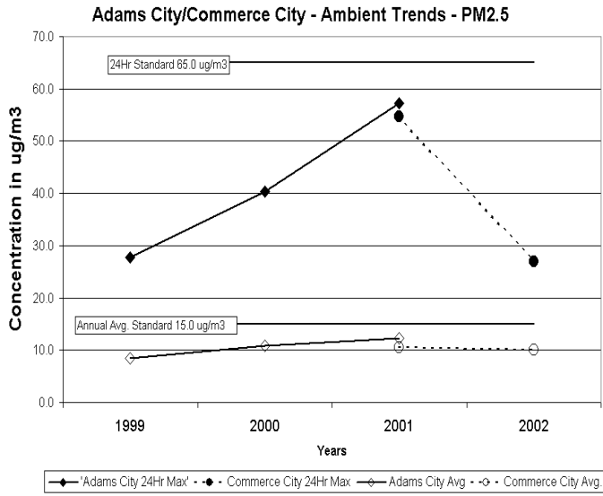
Figure 16 Northern Front Range PM 2.5 Particulate Graphs
