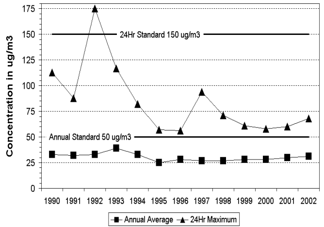
Denver Gates, S. 1050 Broadway - Ambient Trends - PM10
