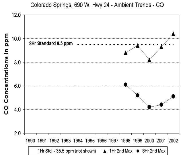
Figure 29 - Southern Front Range Carbon Monoxide Graphs
