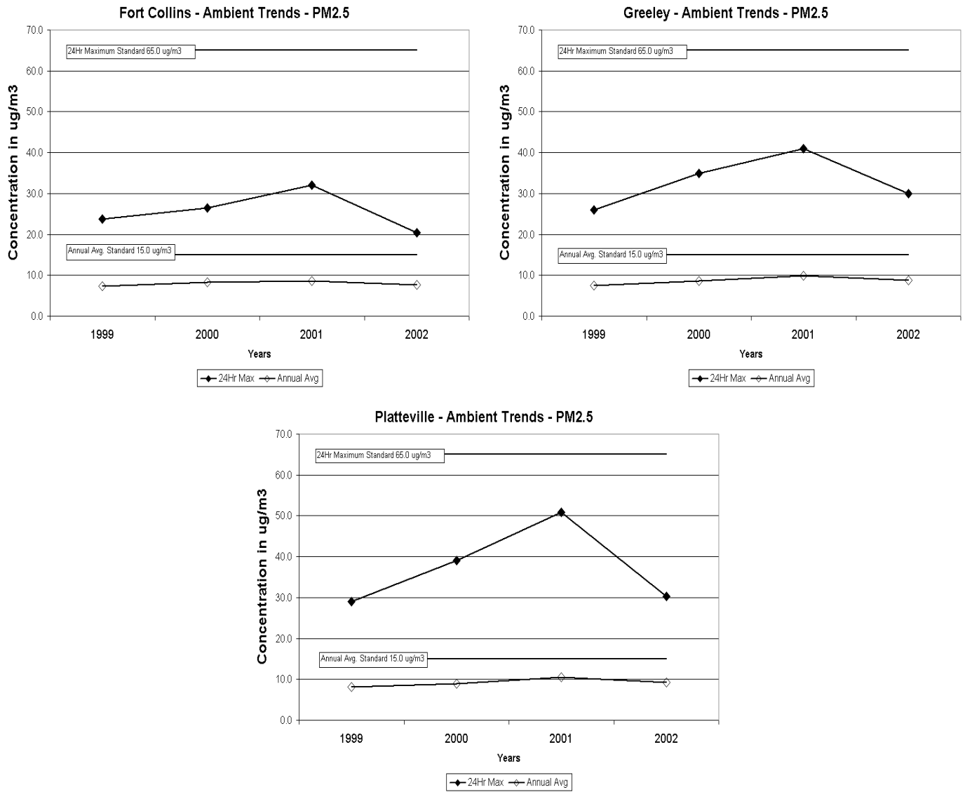
Figure 16- Northern Front Range PM 2.5 Particulate Graphs (continued)
