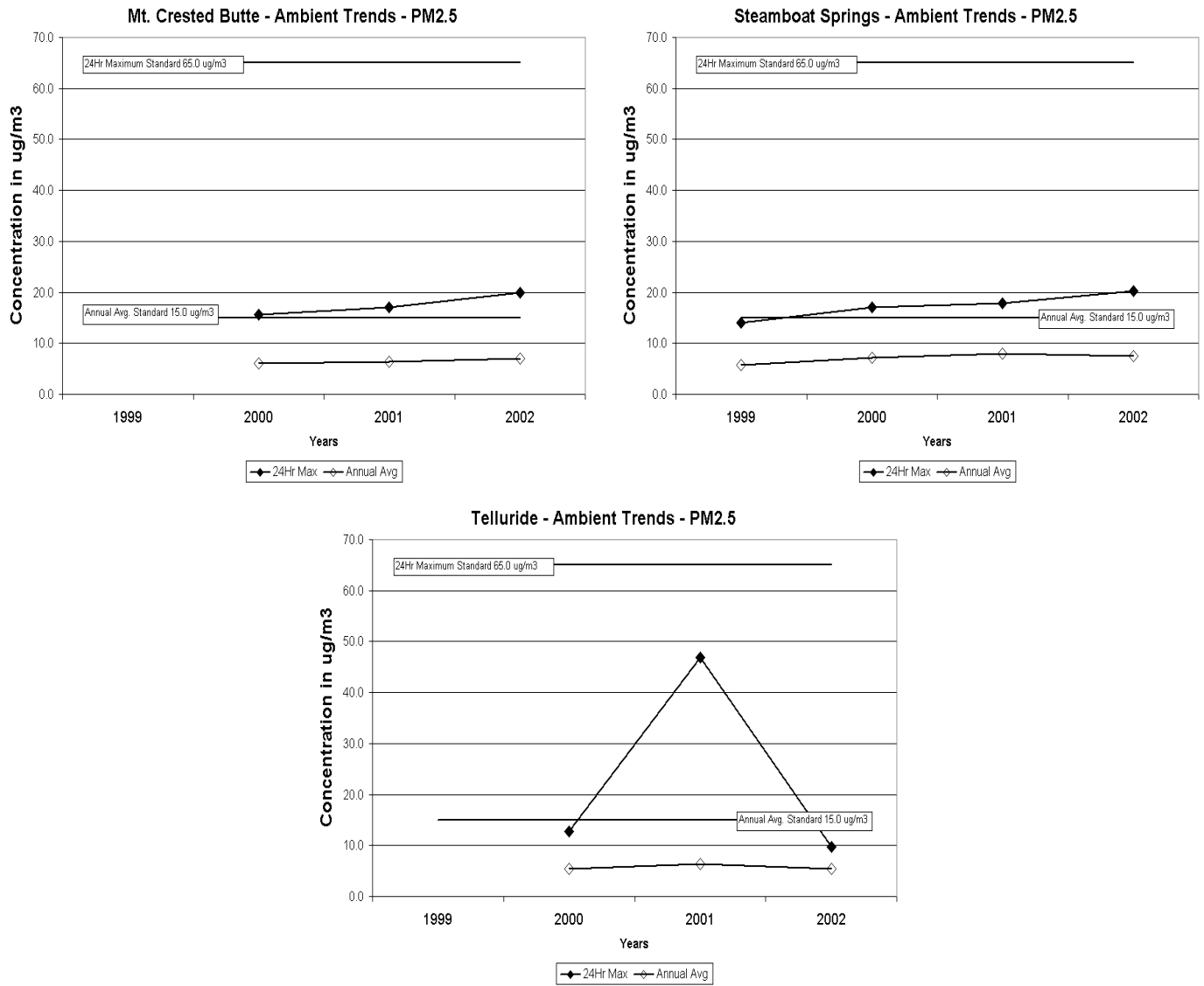
Figure 33 – Mountain Communities PM 2.5 Particulate Graphs
