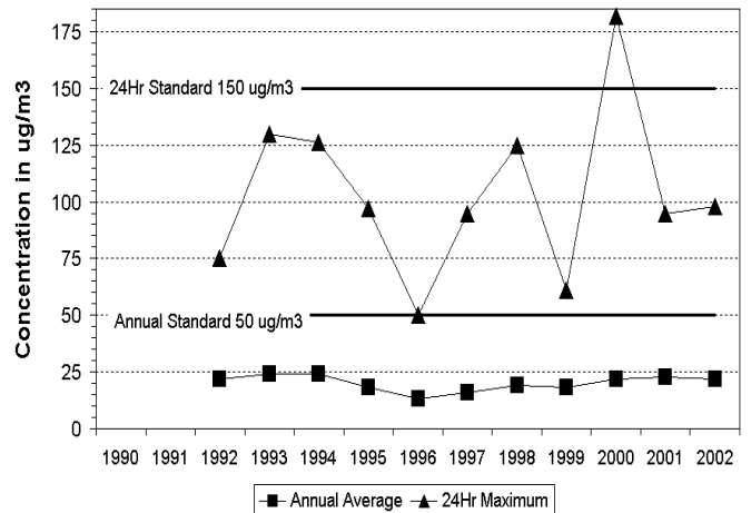
Breckenridge, County Justice Center - Ambient Trends - PM10
