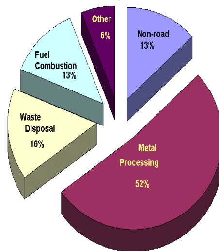
Figure 8 National Emissions by Source Category - 1997 Lead 3,915 tons
