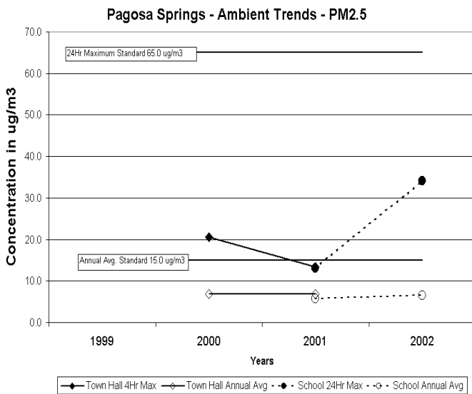
Figure 37 – Western Communities PM 2.5 Particulate Graphs
