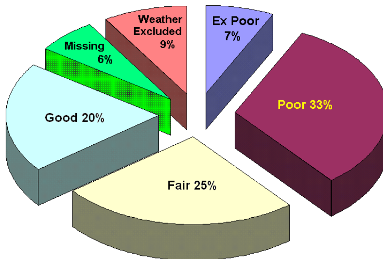
Figure 22 Denver Visibility Data January 2002 - December 2002
