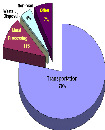
Figure 7 National Emissions by Source Category - 1970 Lead 221,000 tons
