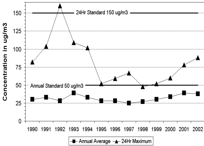
Denver CAMP, 2150 Broadway - Ambient Trends - PM10
