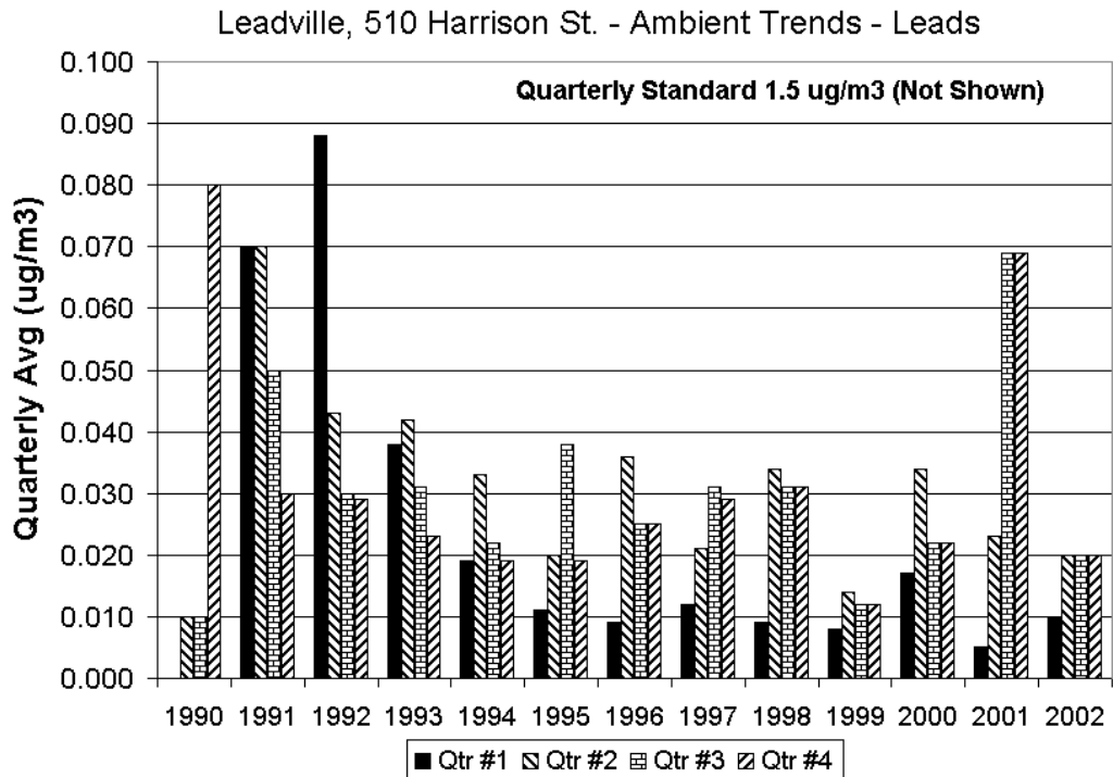
Figure 34 – Mountain Communities Lead Graphs
