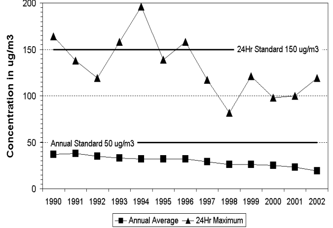
Steamboat Springs, 136 6th St. - Ambient Trends - PM10
