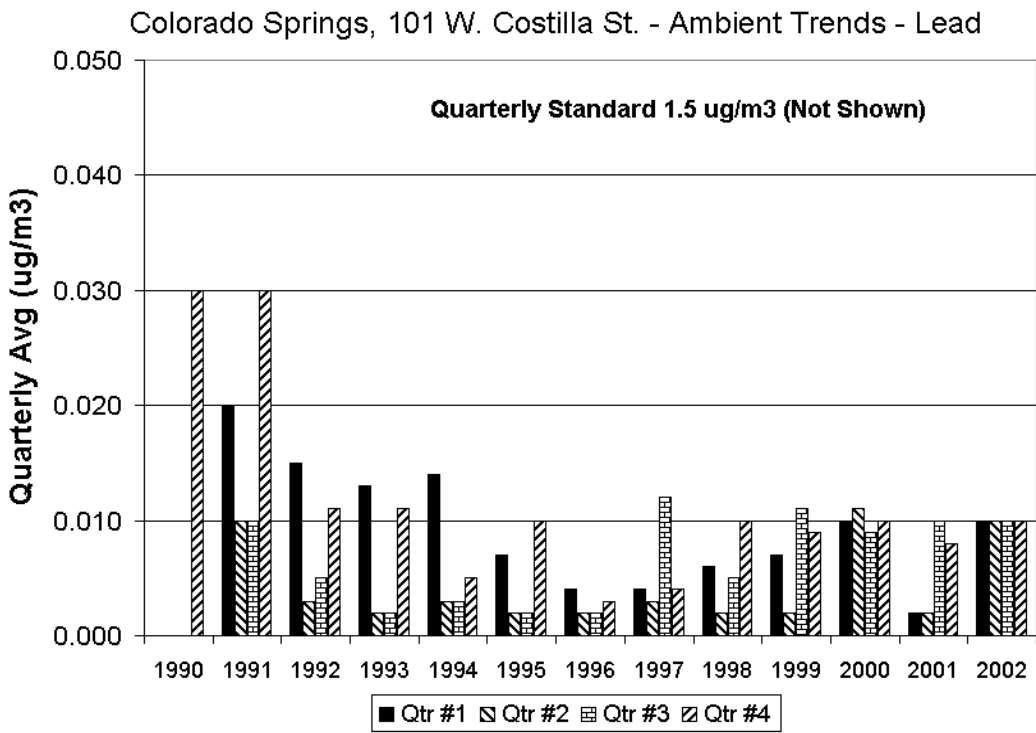
Figure 28 - Southern Front Range Lead Graph
