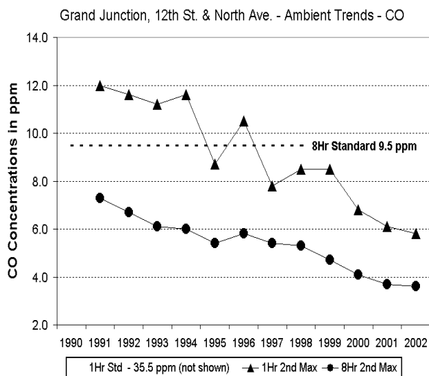
Figure 38 – Western Communities Carbon Monoxide
