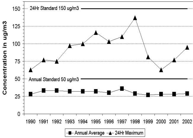
Crested Butte, Colo. 135 & Whiterock - Ambient Trends - PM10
