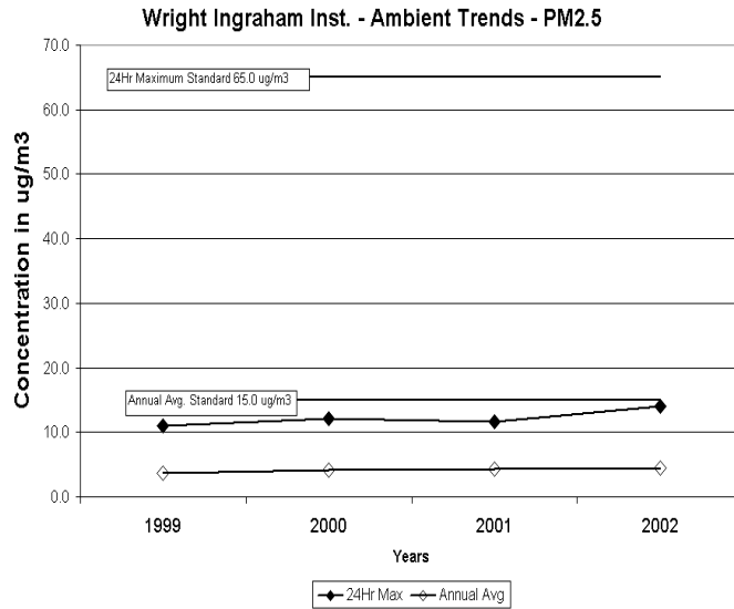
Figure 13- Eastern Plains PM 2.5 Particulate Graphs
