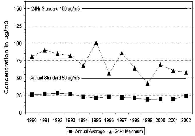
Brighton, 22 4th Ave. - Ambient Trends - PM10
