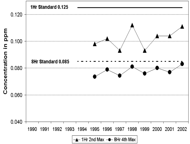
Chatfield Reservoir, Roxborough Pk Rd. - Ambient Trends - Ozone
