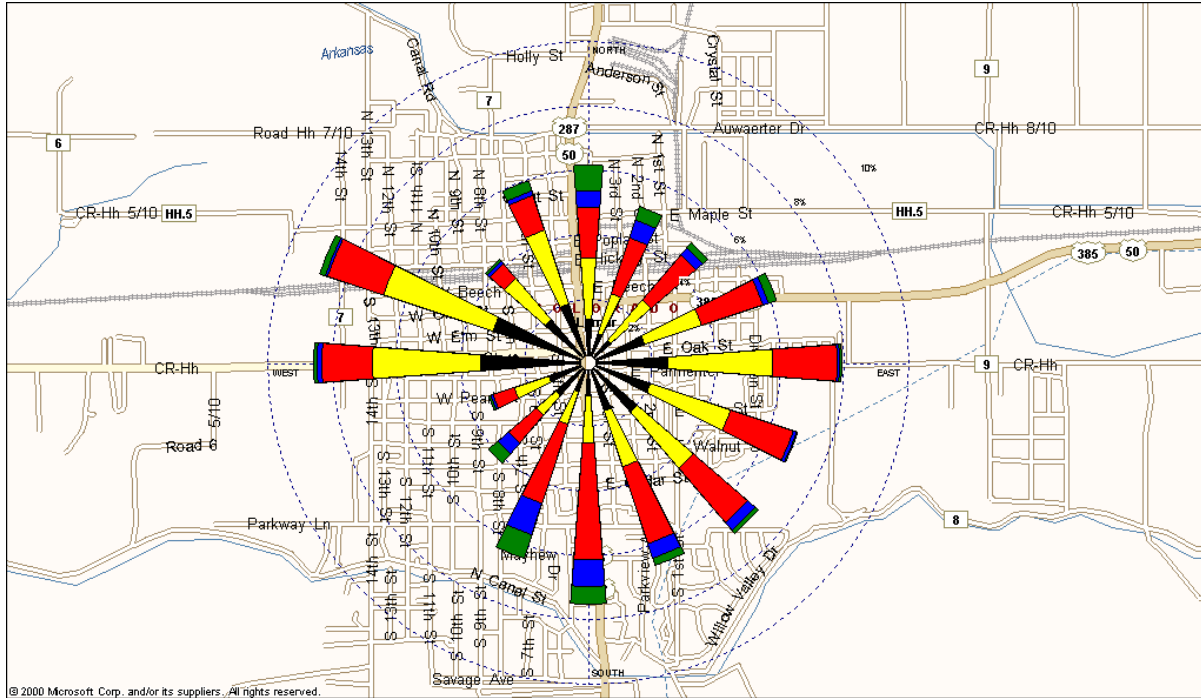
Figure 14- Eastern Plains Wind Rose Lamar, 104 Parmenter Ave.
