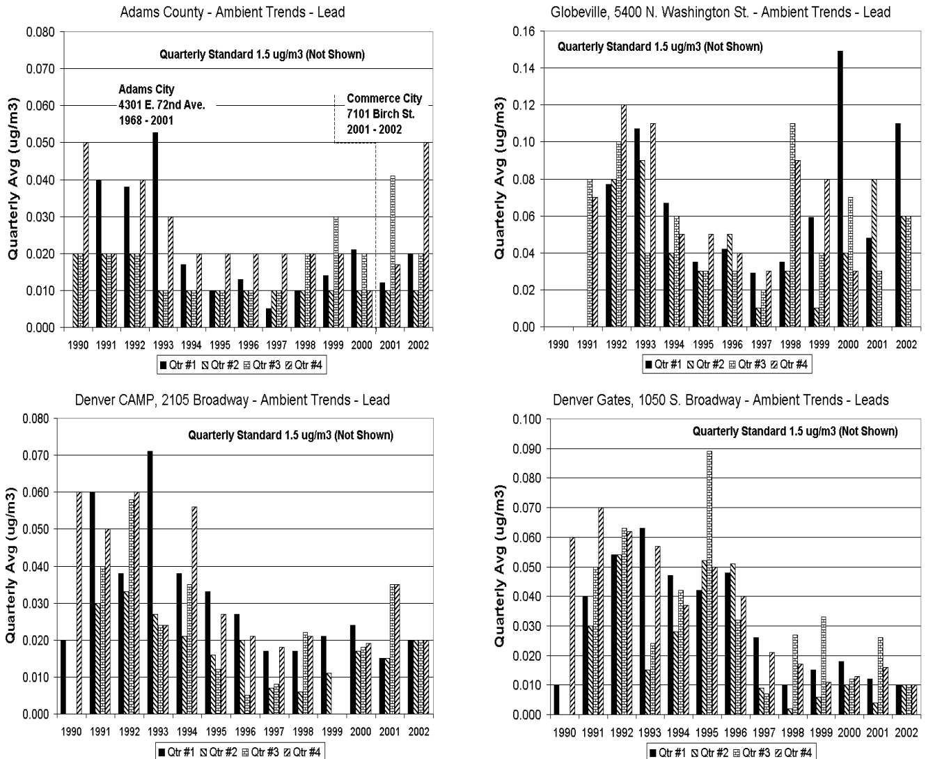
Figure 17- Northern Front Range Lead Graphs
