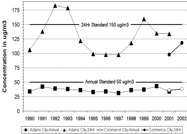
Adams City & Commerce City - Ambient Trends - PM10
