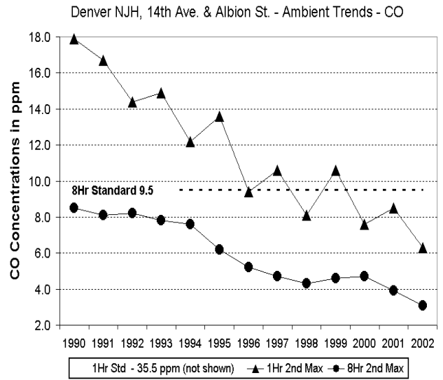
Figure 18- Northern Front Range Carbon Monoxide Graphs (continued)
