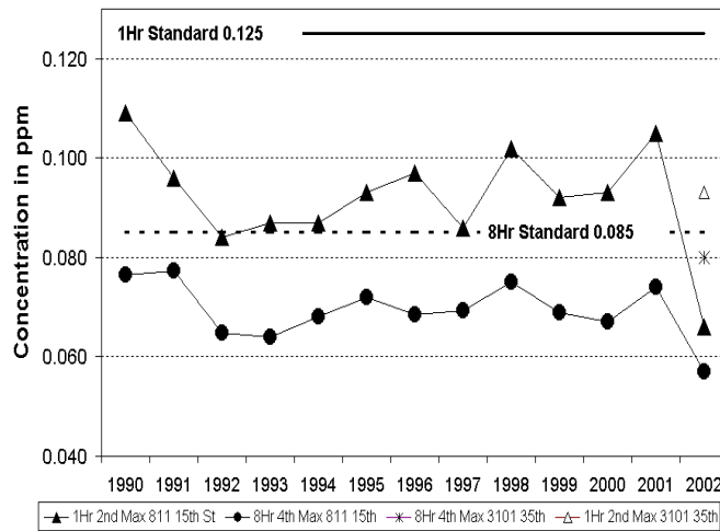
Greeley - Ambient Trends - Ozone
