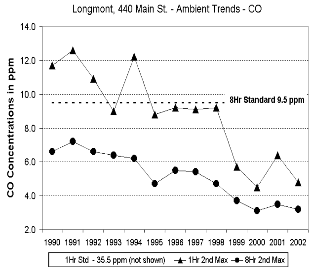
Figure 18- Northern Front Range Carbon Monoxide Graphs
