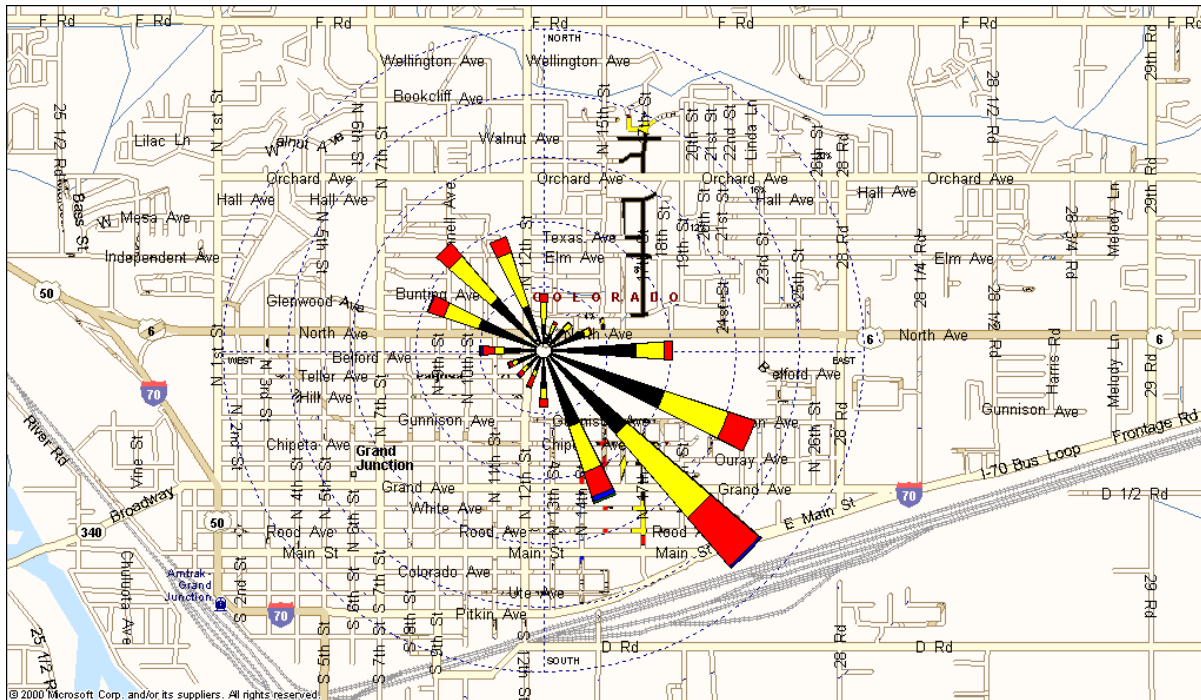
Figure 39 - Western Communities Wind Roses Grand Junction, 12 th St. & North Ave.
