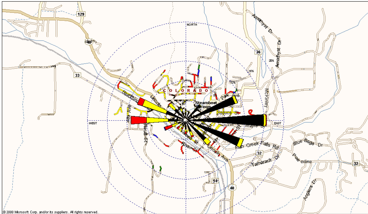
Figure 35 - Mountain Communities Wind Roses Steamboat Springs, 137 10 th St.
