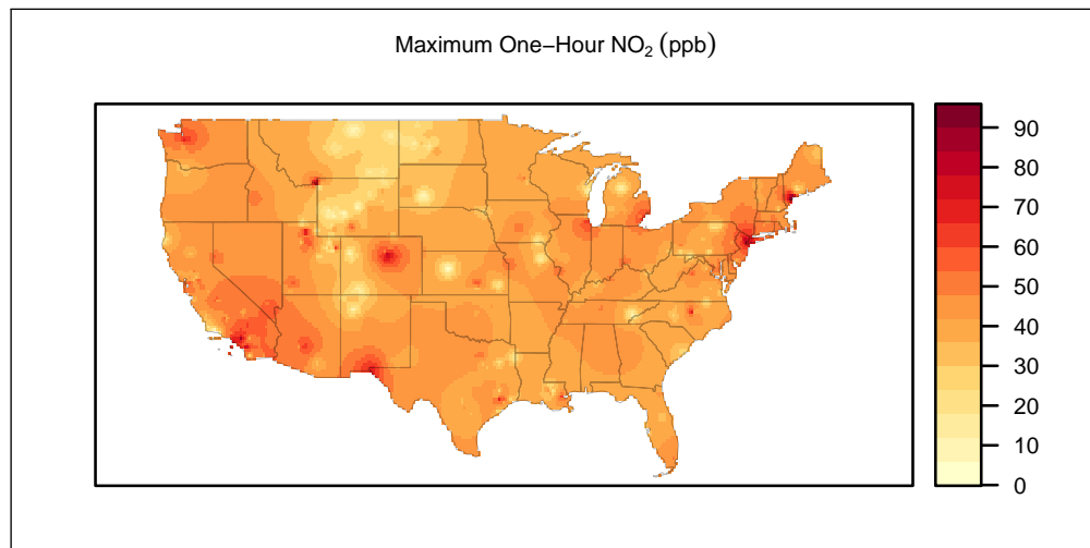
Figure 2.17: Interpolation map of maximum one-hour NO 2 values for air quality monitoring stations in the continental U.S. during 2020
