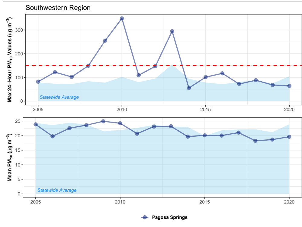
Figure 4.37: Fifteen-year trend in maximum 24-hour PM 10 values (top) and annual mean concentrations (bottom) for monitoring sites in the Southwest region. The 24-hour NAAQS (150 µg m -3 ) is shown as a dashed red line.
