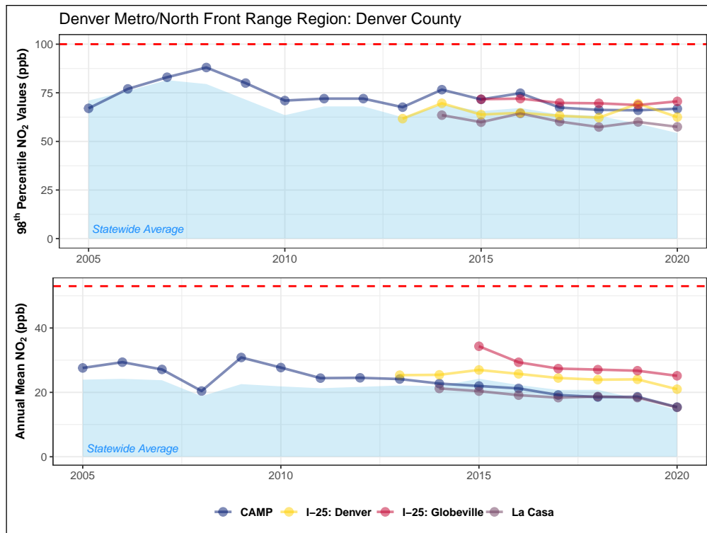
Figure 4.20: Fifteen-year trend in one-hour (top) and annual mean (bottom) nitrogen dioxide NAAQS values for monitoring sites in Denver County. The one-hour and annual mean standards (100 ppb and 53 ppb, respectively) are shown as dashed red lines.
