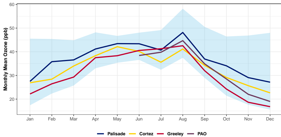
Figure 5.7: Monthly mean ozone concentrations. The blue shaded region shows the statewide range of monthly mean values.
