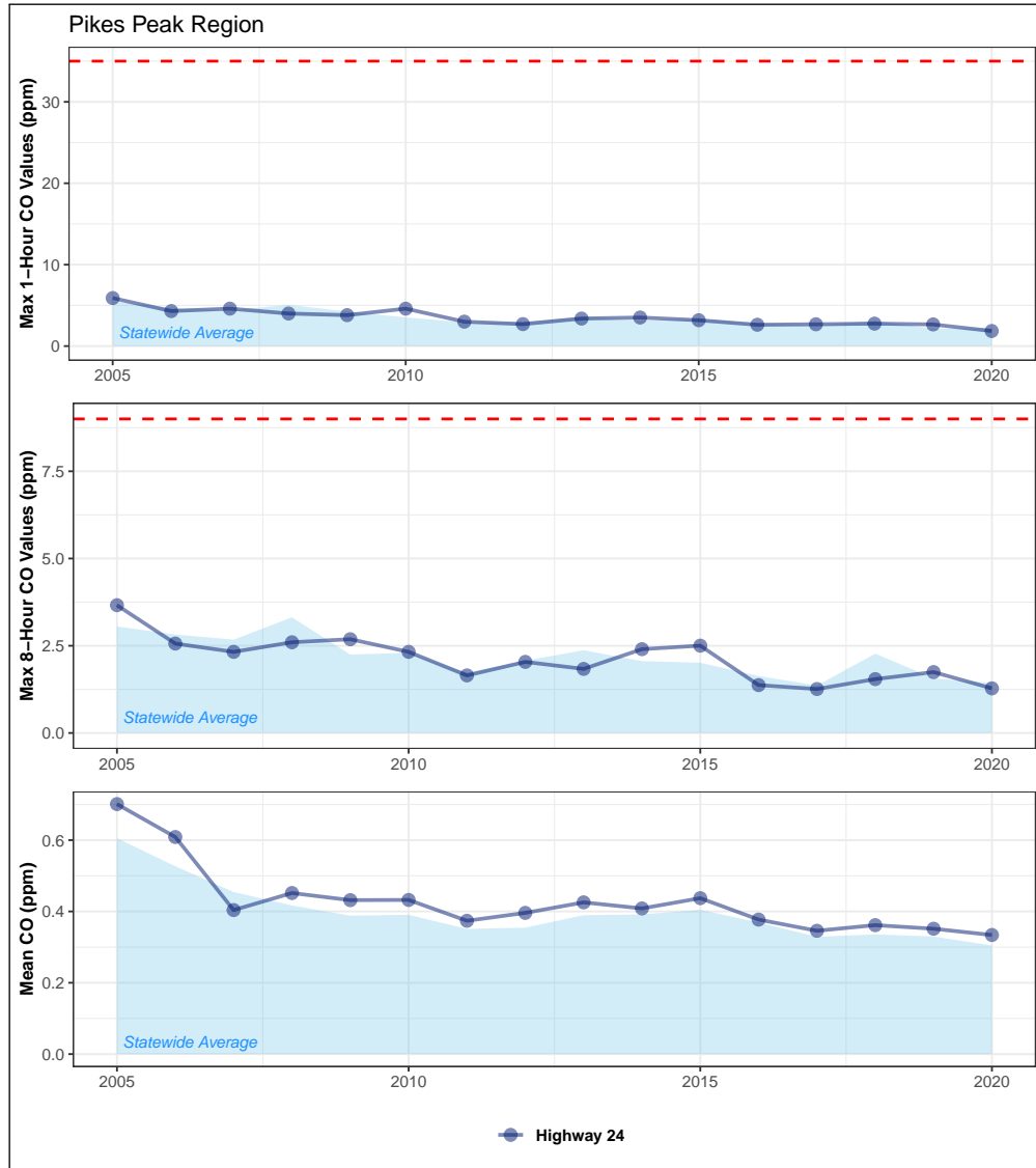
Figure 4.31: Fifteen-year trend in annual maximum one-hour (top) and eight-hour (center) CO values and annual mean eight-hour CO concentrations (bottom) for monitoring sites in the Pikes Peak region. The one-hour and eight-hour NAAQS (35 ppm and 9 ppm, respectively) are shown as dashed red lines.
