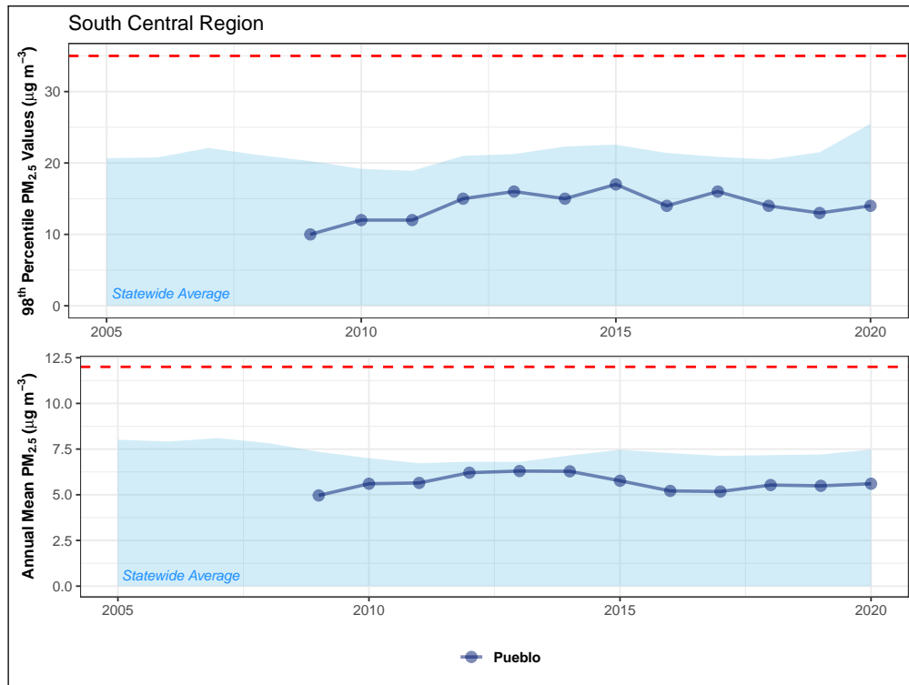
Figure 4.36: Fifteen-year trend in 24-hour PM 2.5 annual 98 th percentile values (top) and annual mean concentrations (bottom) for monitoring sites in the South Central region. The 24-hour and annual mean NAAQS (35 µg m -3 and 12 µg m -3 , respectively) are shown as dashed red lines.
