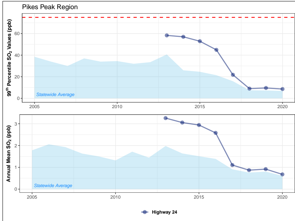
Figure 4.33: Fifteen-year trend in sulfur dioxide one-hour NAAQS values (top) and annual mean one-hour concentrations (bottom) for monitoring sites in the Pikes Peak region. The one-hour NAAQS (75 ppb) is shown as a dashed red line.
