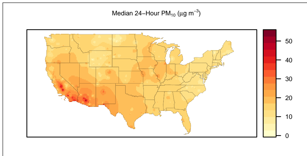
Figure 2.21: Interpolation map of median 24-hour PM 10 values for air quality monitoring stations in the continental U.S. during 2020
