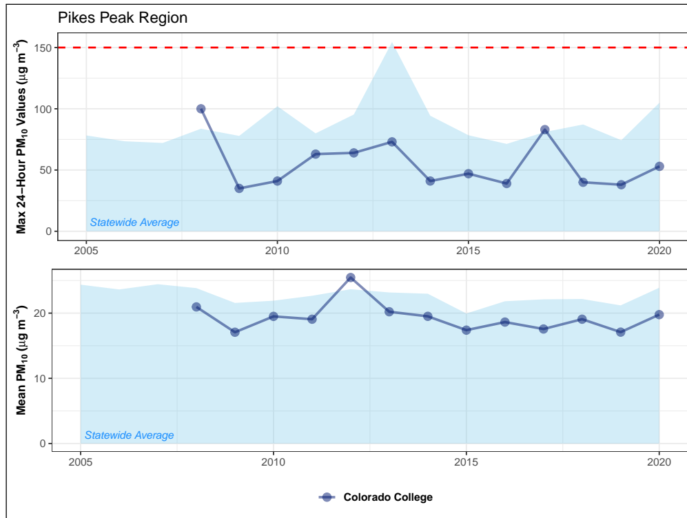
Figure 4.29: Fifteen-year trend in maximum 24-hour PM 10 values (top) and annual mean concentrations (bottom) for monitoring sites in the Pikes Peak region. The 24-hour NAAQS (150 µg m -3 ) is shown as a dashed red line.
