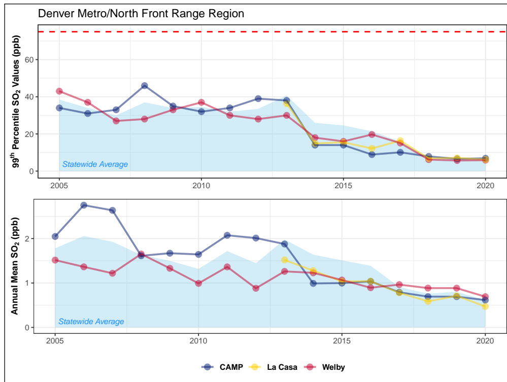
Figure 4.23: Fifteen-year trend in sulfur dioxide one-hour NAAQS values (top) and annual mean one-hour concentrations (bottom) for monitoring sites in the Denver Metro/Northern Front Range region. The one-hour NAAQS (75 ppb) is shown as a dashed red line.
