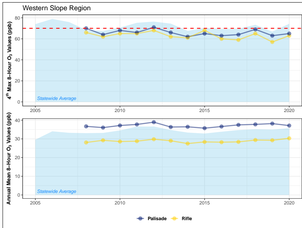
Figure 4.41: Fifteen-year trend in ozone eight-hour NAAQS values (top) and annual mean eight-hour concentrations (bottom) for monitoring sites in the Western Slope region. The eight-hour NAAQS (70 ppb) is shown as a dashed red line.
