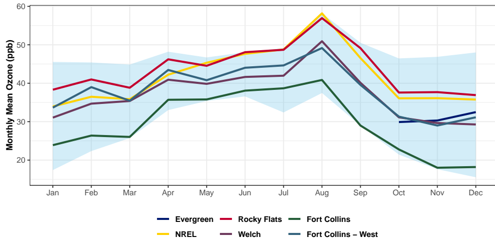
Figure 5.6: Monthly mean ozone concentrations. The blue shaded region shows the statewide range of monthly mean values.
