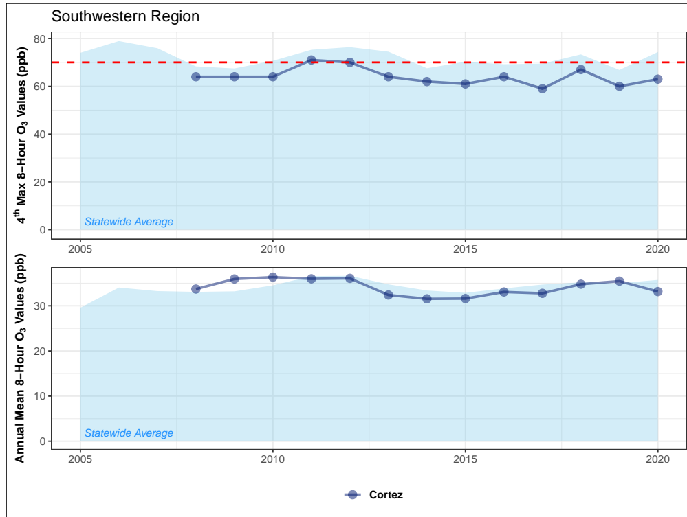
Figure 4.38: Fifteen-year trend in ozone eight-hour NAAQS values (top) and annual mean eight-hour concentrations (bottom) for monitoring sites in the Southwest region. The eight-hour NAAQS (70 ppb) is shown as a dashed red line.
