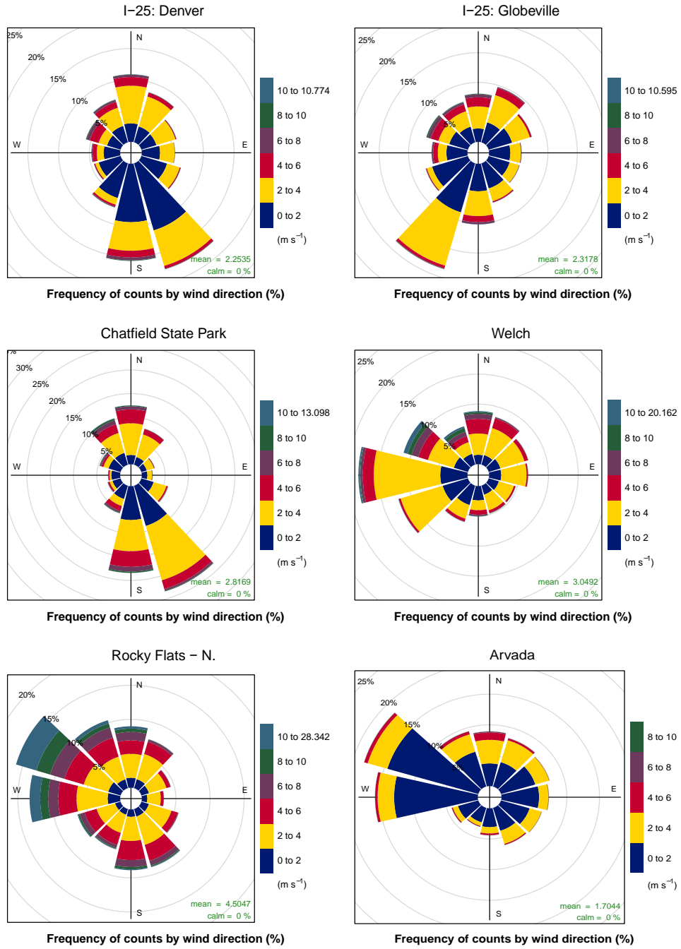
Figure 4.26: Wind roses for sites in the Denver Metro/North Front Range Region during 2020 (continued).
