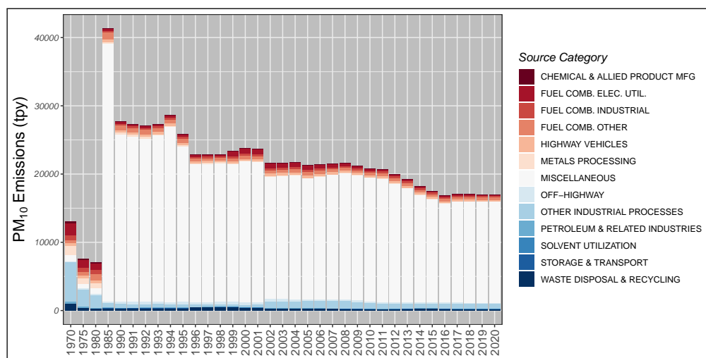
Figure 2.18: Trends in national \text{PM}_{10} emissions from 1970 to 2020.
