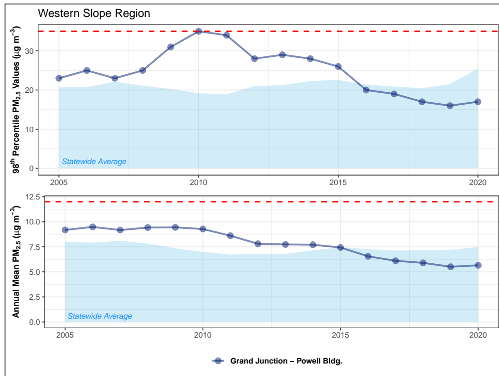
Figure 4.40: Fifteen-year trend in 24-hour PM 2.5 annual 98 th percentile values (top) and annual mean concentrations (bottom) for monitoring sites in the Western Slope region. The 24-hour and annual mean NAAQS (35 µg m -3 and 12 µg m -3 , respectively) are shown as dashed red lines.
