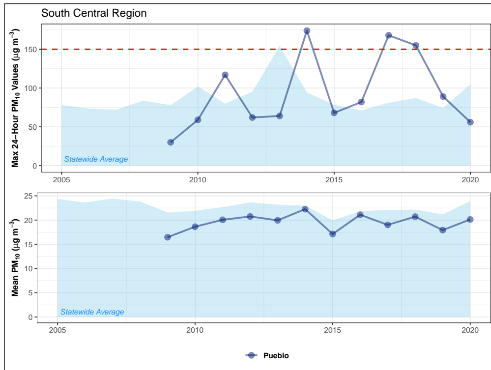
Figure 4.35: Fifteen-year trend in maximum 24-hour PM 10 values (top) and annual mean concentrations (bottom) for monitoring sites in the South Central region. The 24-hour NAAQS (150 µg m -3 ) is shown as a dashed red line.
