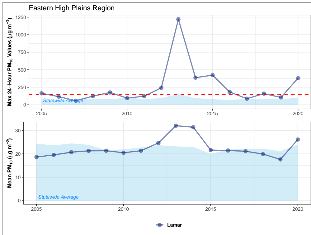
Figure 4.28: Fifteen-year trend in maximum 24-hour PM 10 values (top) and annual mean concentrations (bottom) for monitoring sites in the Eastern High Plains region. The 24-hour NAAQS (150 µg m -3 ) is shown as a dashed red line.
