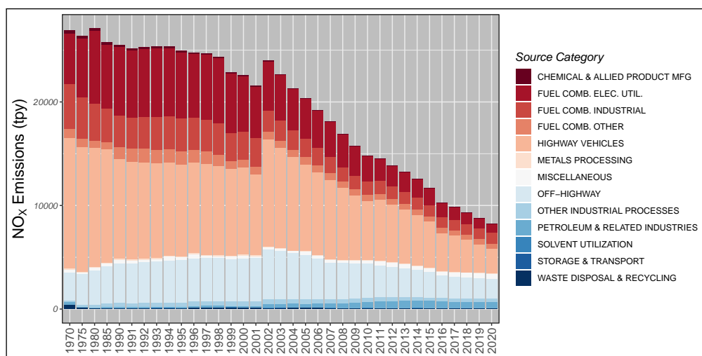
Figure 2.13: Trends in national NO x emissions from 1970 to 2020.
