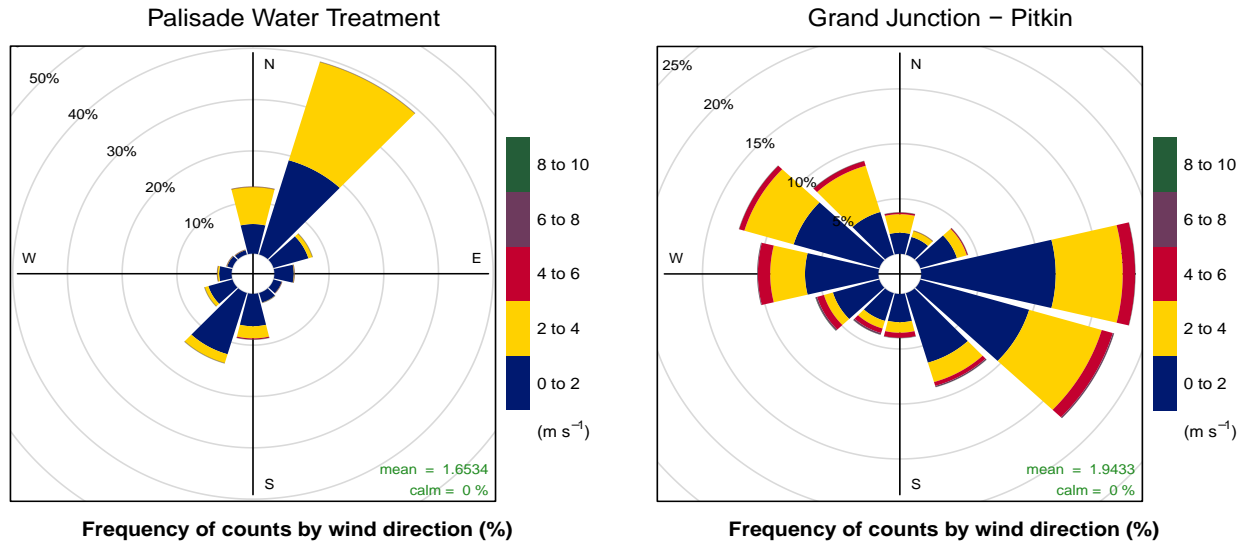
Figure 4.42: Wind roses for sites in the Western Slope Region during 2020.
