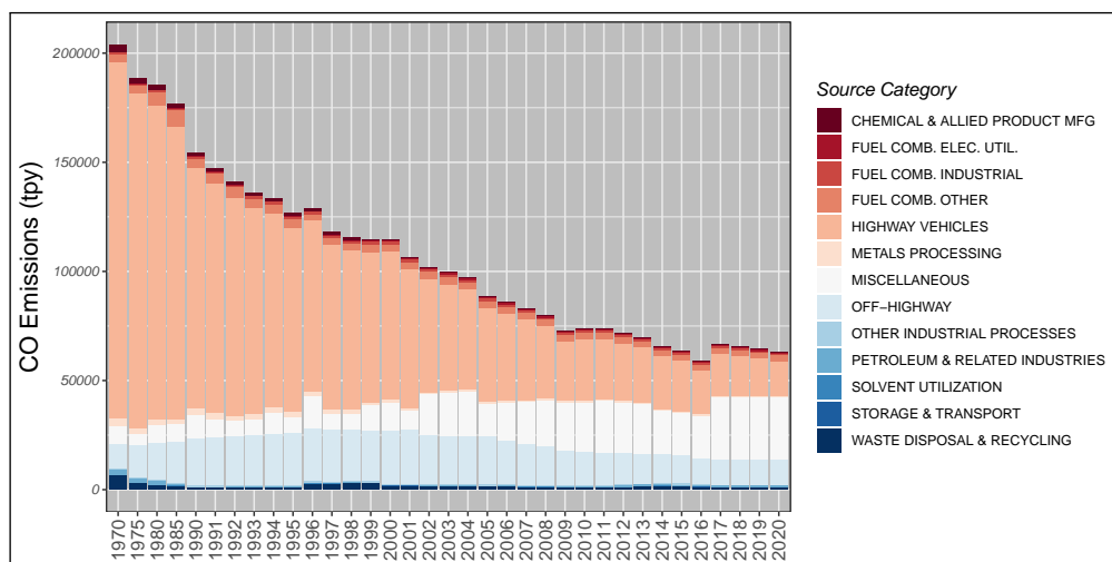
Figure 2.1: Trends in national carbon monoxide emissions from 1970 to 2020.
