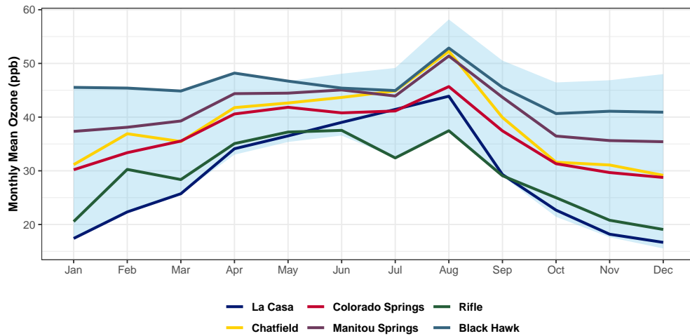
Figure 5.5: Monthly mean ozone concentrations. The blue shaded region shows the statewide range of monthly mean values.
