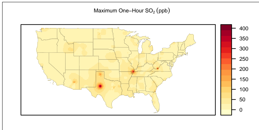
Figure 2.9: Interpolation map of maximum one-hour SO 2 values for air quality monitoring stations in the continental U.S. during 2020
