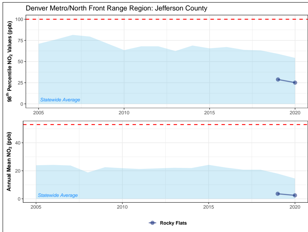
Figure 4.21: Fifteen-year trend in one-hour (top) and annual mean (bottom) nitrogen dioxide NAAQS values for monitoring sites in Jefferson County. The one-hour and annual mean standards (100 ppb and 53 ppb, respectively) are shown as dashed red lines.
