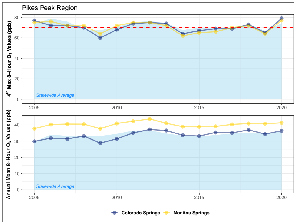
Figure 4.32: Fifteen-year trend in ozone eight-hour NAAQS values (top) and annual mean eight-hour concentrations (bottom) for monitoring sites in the Pikes Peak region. The eight-hour NAAQS (70 ppb) is shown as a dashed red line.
