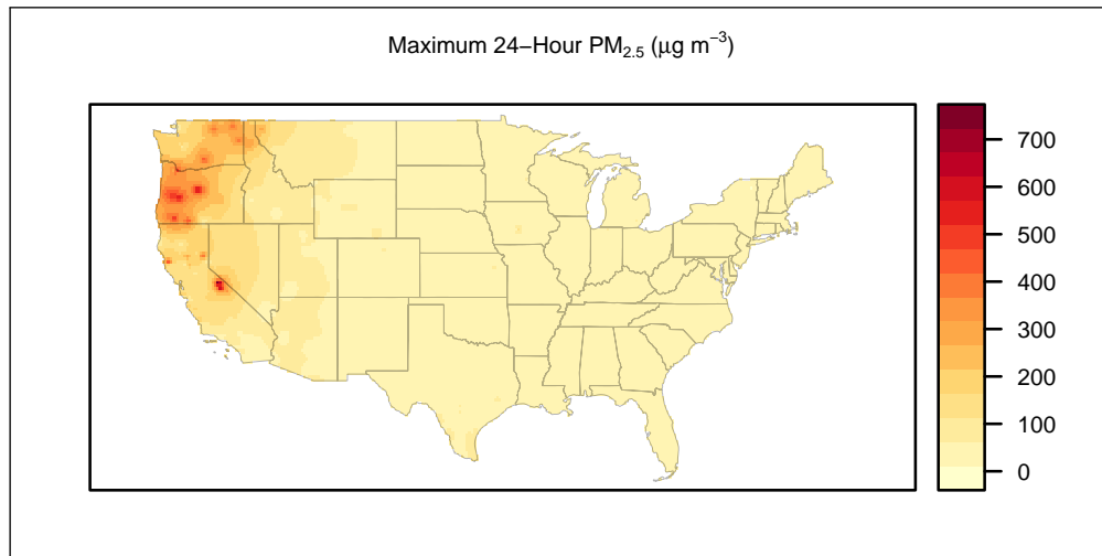
Figure 2.24: Interpolation map of maximum 24-hour PM 2.5 values for air quality monitoring stations in the continental U.S. during 2020
