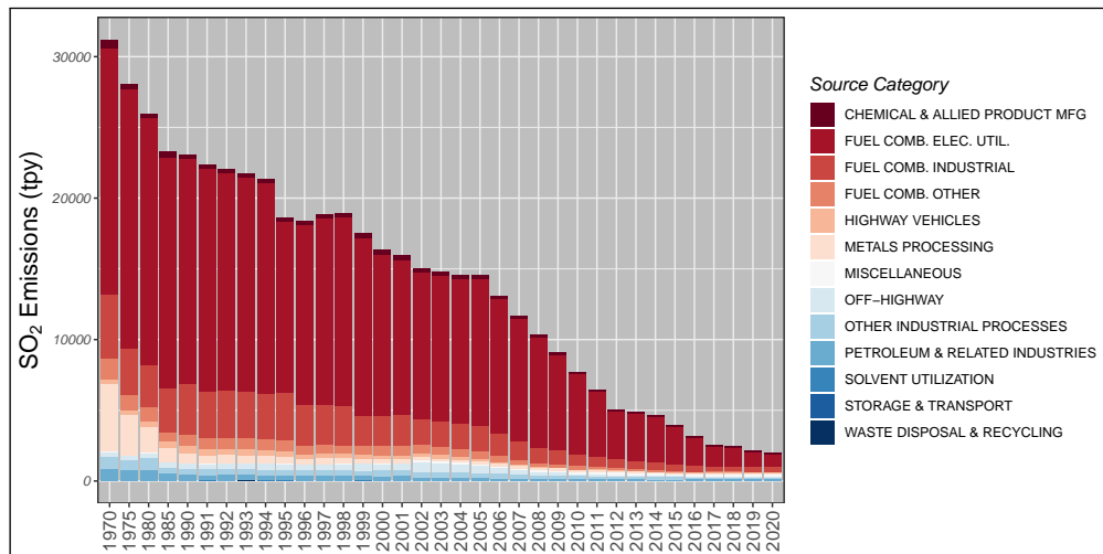
Figure 2.6: Trends in national sulfur dioxide emissions from 1970 to 2020.
