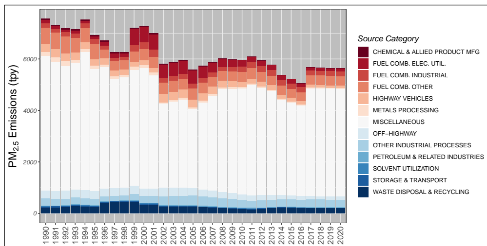
Figure 2.19: Trends in national PM 2.5 emissions from 1990 to 2020.
