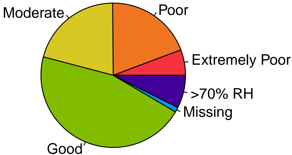
Figure 4.24: Denver visibility data.
