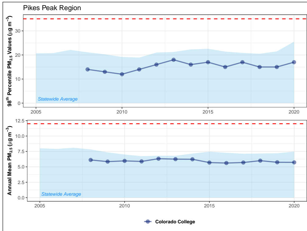
Figure 4.30: Fifteen-year trend in 24-hour PM 2.5 annual 98 th percentile values (top) and annual mean concentrations (bottom) for monitoring sites in the Pikes Peak region. The 24-hour and annual mean NAAQS (35 µg m -3 and 12 µg m -3 , respectively) are shown as dashed red lines.
