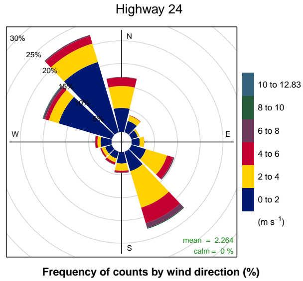
Figure 4.34: Wind rose from the Highway 24 meteorological station.
