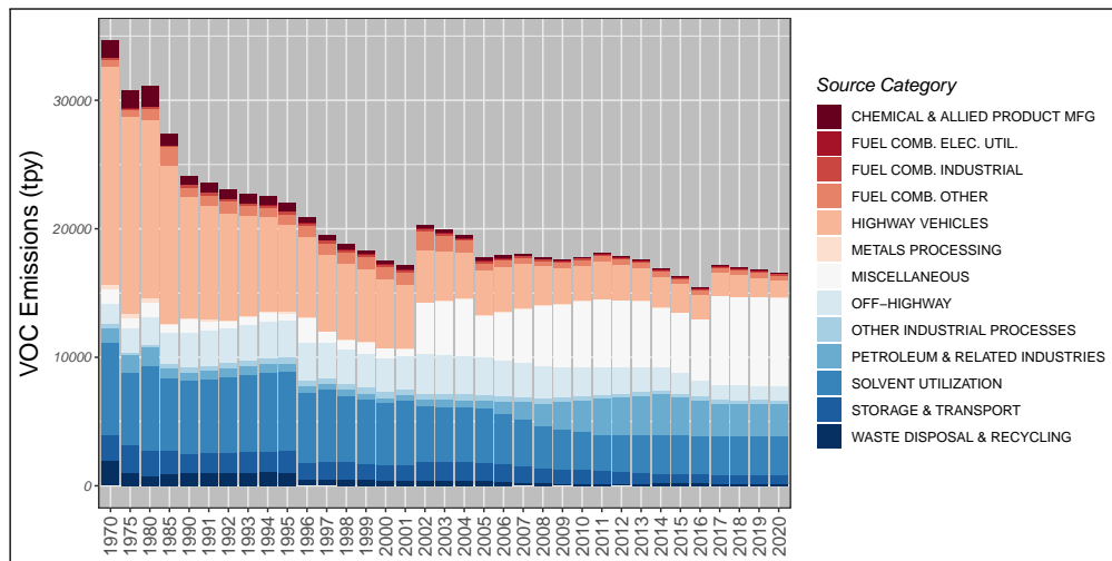
Figure 2.10: Trends in national VOC emissions from 1970 to 2020.
