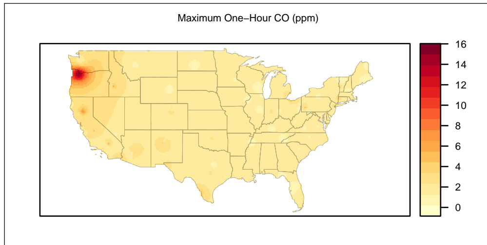
Figure 2.5: Interpolation map of maximum one-hour CO values for air quality monitoring stations in the continental U.S. during 2020
