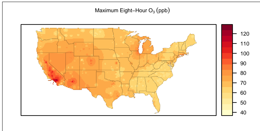
Figure 2.12: Interpolation map of maximum eight-hour O 3 values for air quality monitoring stations in the continental U.S. during 2020
