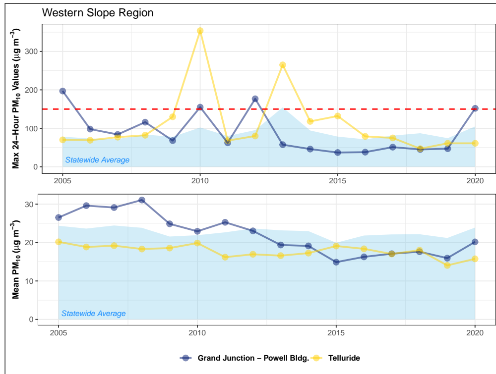
Figure 4.39: Fifteen-year trend in maximum 24-hour PM 10 values (top) and annual mean concentrations (bottom) for monitoring sites in the Western Slope region. The 24-hour NAAQS (150 µg m -3 ) is shown as a dashed red line.
