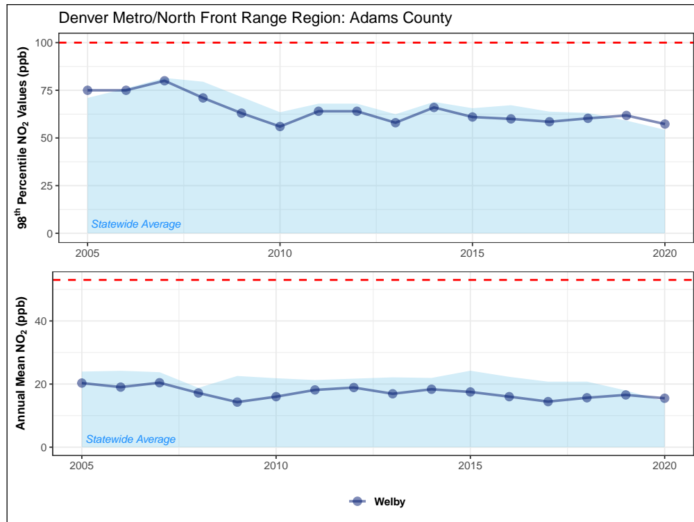
Figure 4.19: Fifteen-year trend in one-hour (top) and annual mean (bottom) nitrogen dioxide NAAQS values for monitoring sites in Adams County. The one-hour and annual mean standards (100 ppb and 53 ppb, respectively) are shown as dashed red lines.
