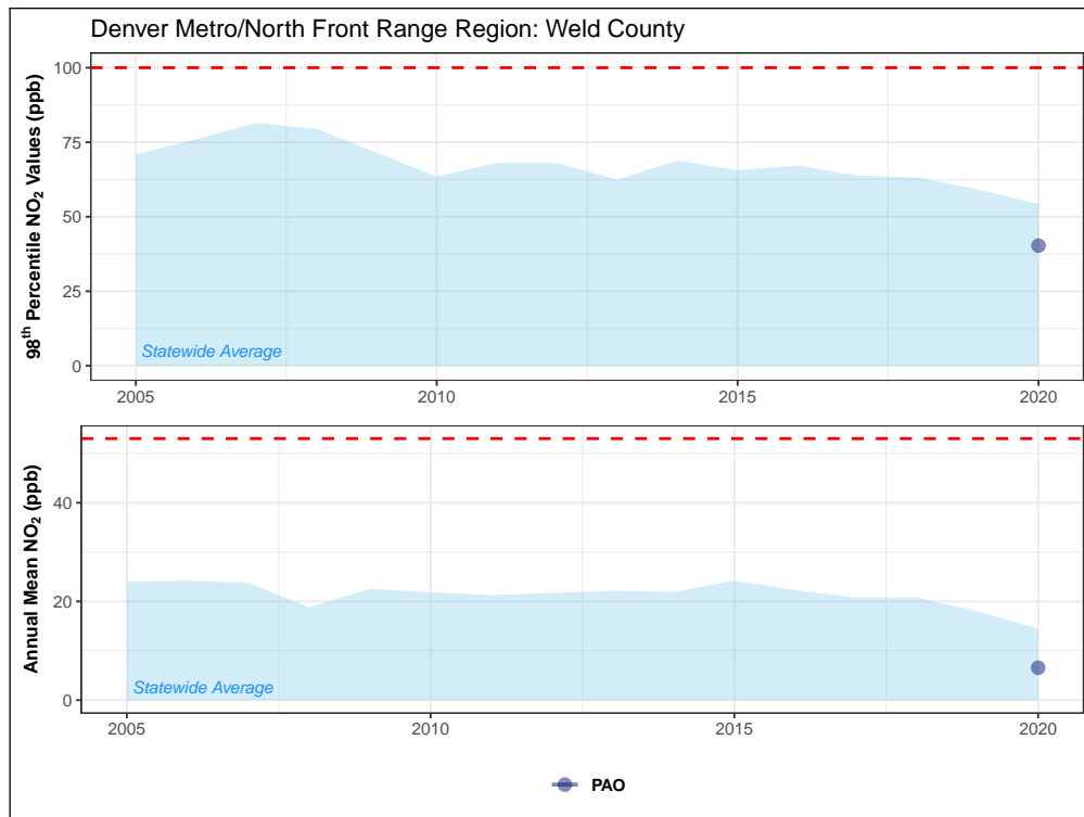
Figure 4.22: Fifteen-year trend in one-hour (top) and annual mean (bottom) nitrogen dioxide NAAQS values for monitoring sites in Weld County. The one-hour and annual mean standards (100 ppb and 53 ppb, respectively) are shown as dashed red lines.
