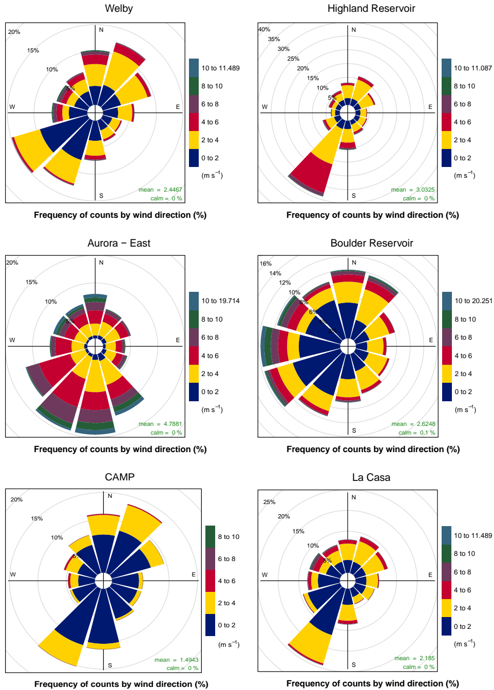
Figure 4.25: Wind roses for sites in the Denver Metro/North Front Range Region during 2020.
